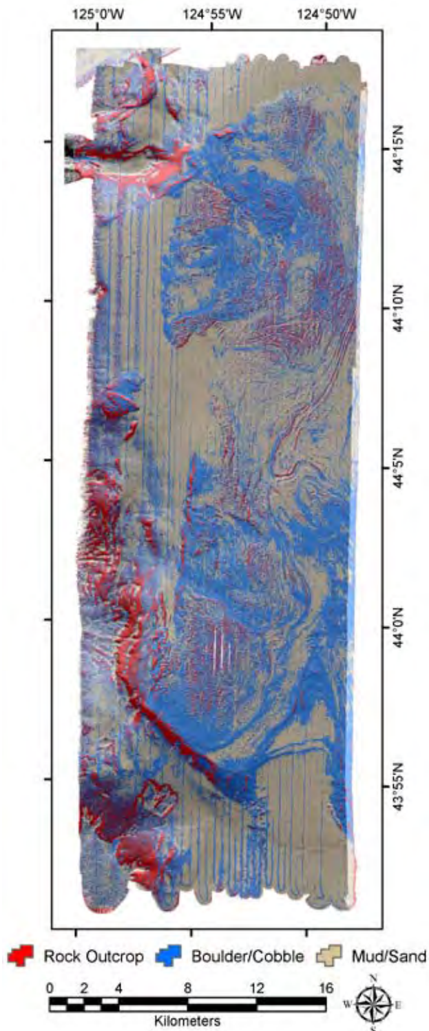
Figure 4. Habitat classification scheme for Heceta Bank integrating submersible and multibeam data (after Whitmire et al. 2007).
